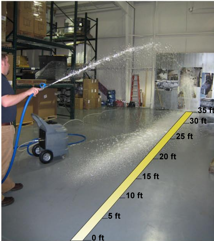
Horizontal Throw with FloJet Pump (35 ft or 11 M)
